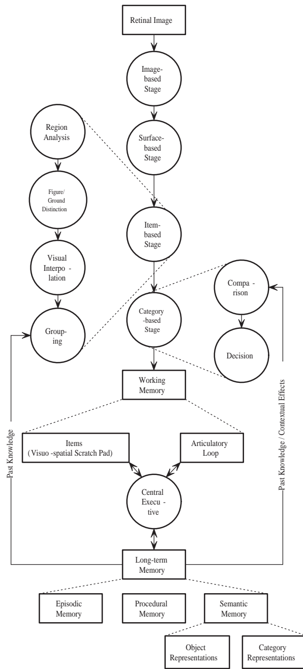
Figure 2: Theory 3 of program comprehension through vision.
