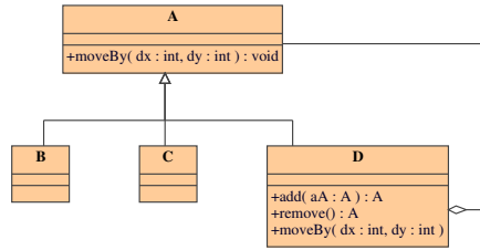
Figure 1: What is the structure and function that an expert software engineer recognises instantly in this subset of a UML class diagram of a well-known program and that a novice software engineer does not? How does the recognition happen?
