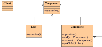
Figure 4: Original class diagram of the Composite design pattern [13, p. 163].
