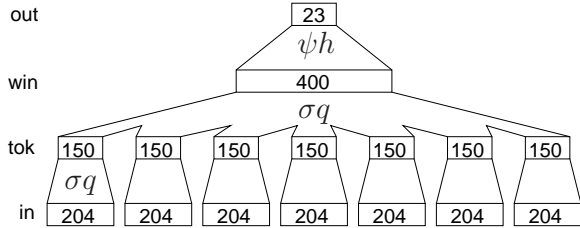
Figure 1: Illustration of our baseline I-T-W-O model (see Secs. 4 and 5.1). The input layer comprises seven tokens with 204 dimensions each. Each token is passed through a shared 150-dimensional token feature extractor. These 7 \cdot 150 features are concatenated and 400 features are extracted from them in the window layer. These 400 features are the input to the final 23-class output prediction. Feature extractors \sigma q and \psi h are described in Section 3.
